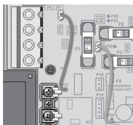
Connections for all 240 V heaters (North American installations only)
