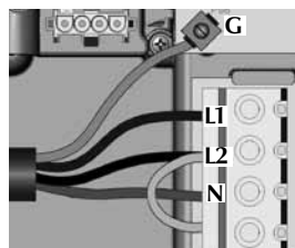
2-phases with single neutral
