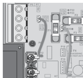
Connections for all 120 V heaters (North American installation in.ye-3 only)
