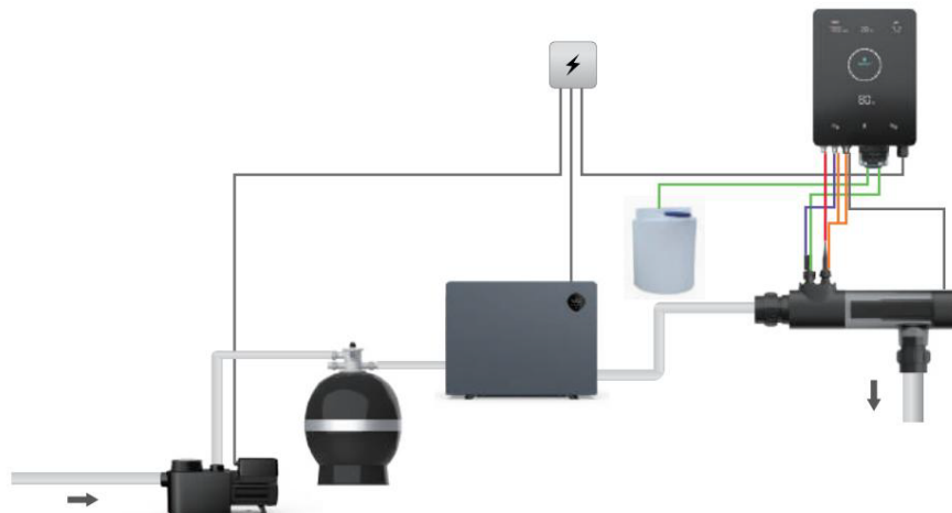
1: Installationsdiagram
